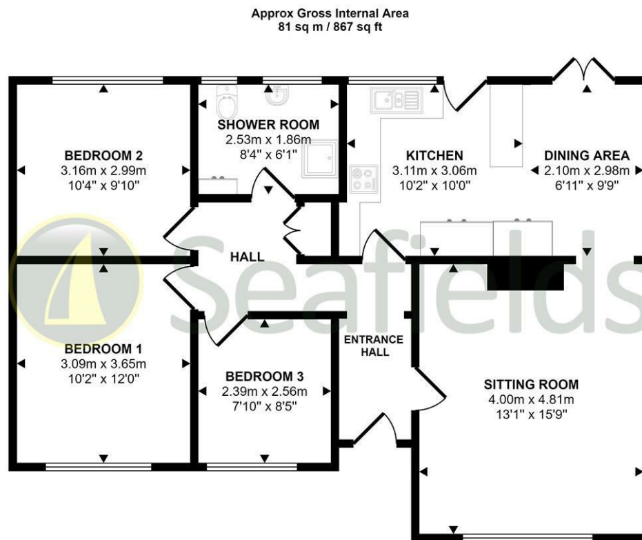
Floorplan
